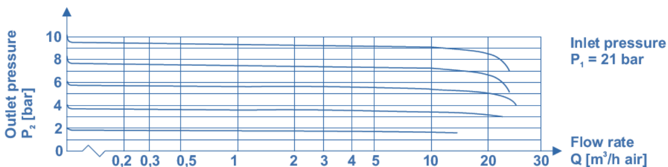
Flow curves BM56-1
